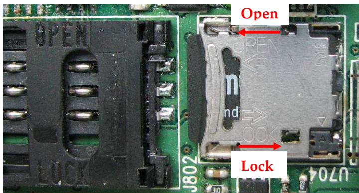
Micro SD card inserted and locked
